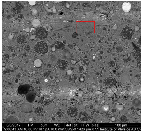
Figure 5: Microstructure of AAFA (rectangle shows a N-A-S-H gel region).
