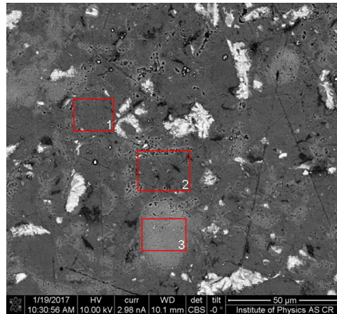
Figure 4: Microstructure of cement paste (1=inner product with C-S-H HD , 2=outer product with C-S-H LD , 3=CH).
