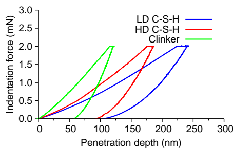
Figure 1: Typical load-displacement nanoindentation curves on cement paste.
