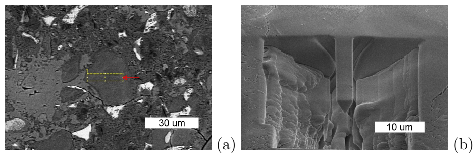
Figure 19: Cantilever micro-beam fabricated in the inner product. (a) Location before FIB milling labeled by the yellow rectangle. The red arrow indicates the fixed end position. (b) Front view of the cantilever after FIB milling. After [10].
